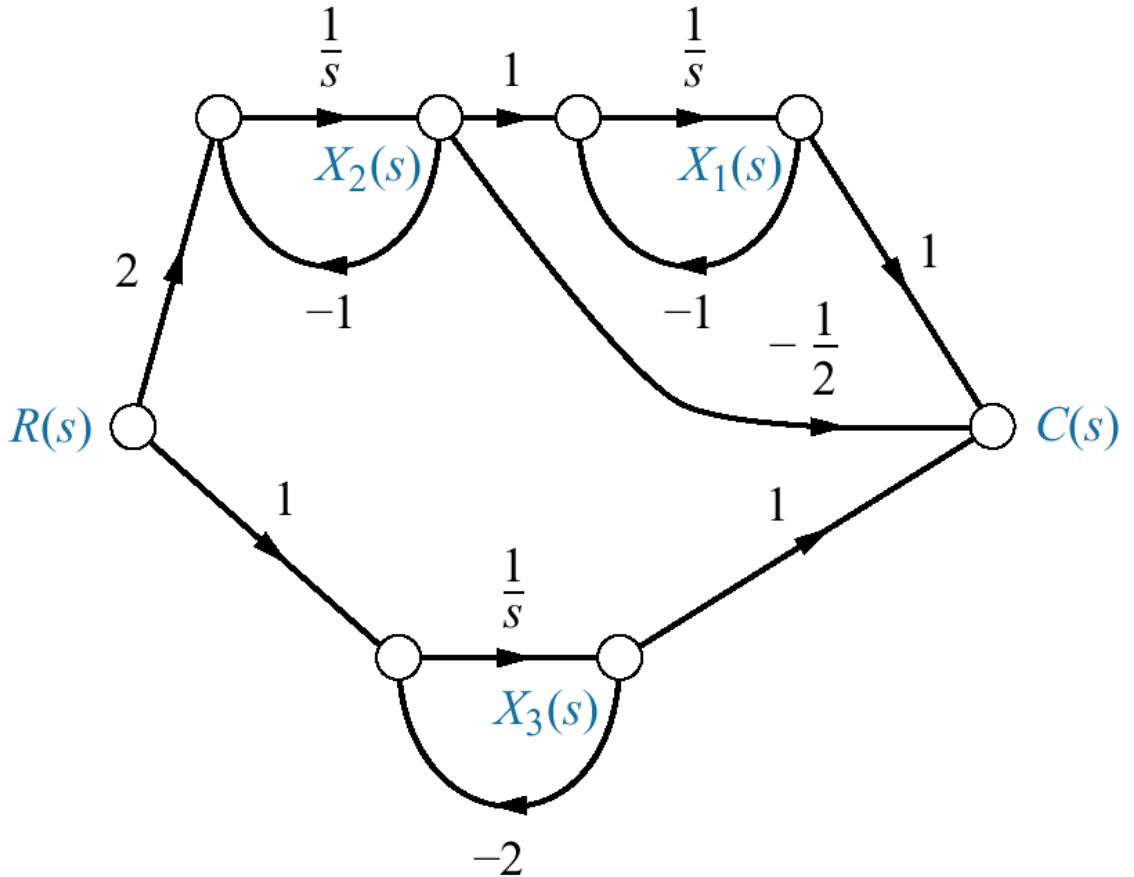
Figure 5.26 Signal-flow representat ion of Eq. (5.52)
