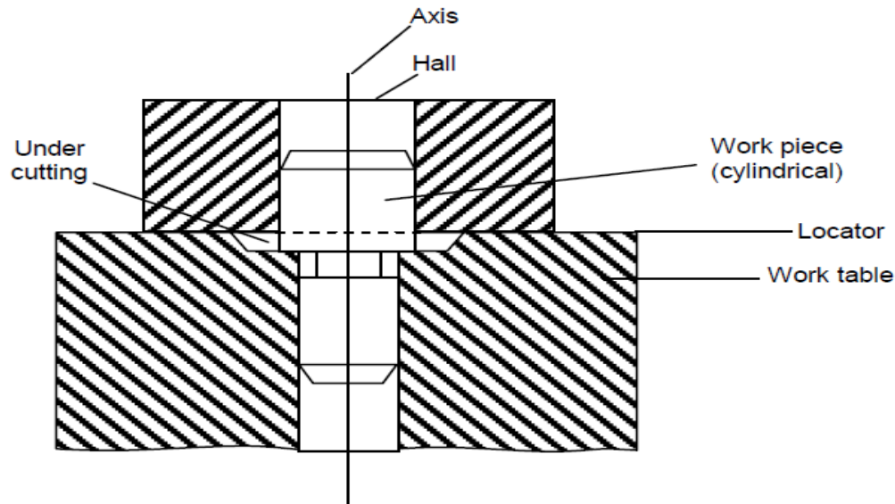
Figure 4.4 : Cylindrical Locator
