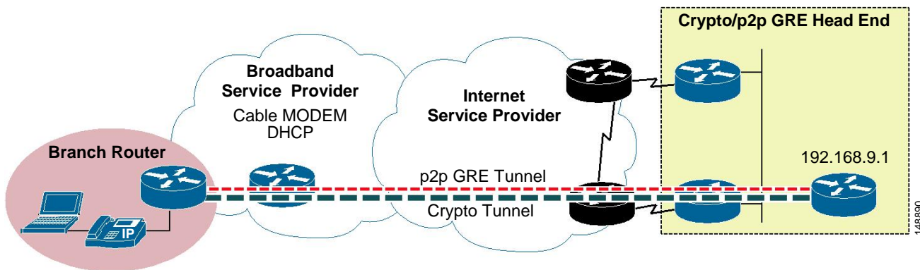
Figure 5-1 Sample Topology
