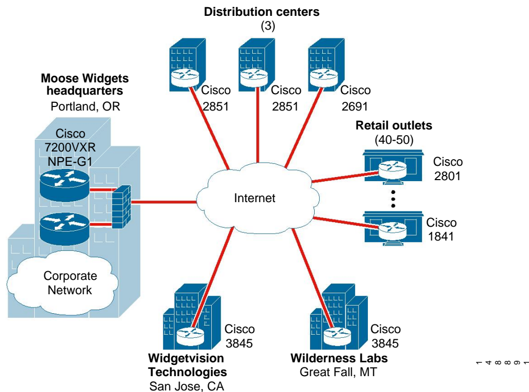
Figure 5-3 Moose Widgets Case Study—VPN Topology
