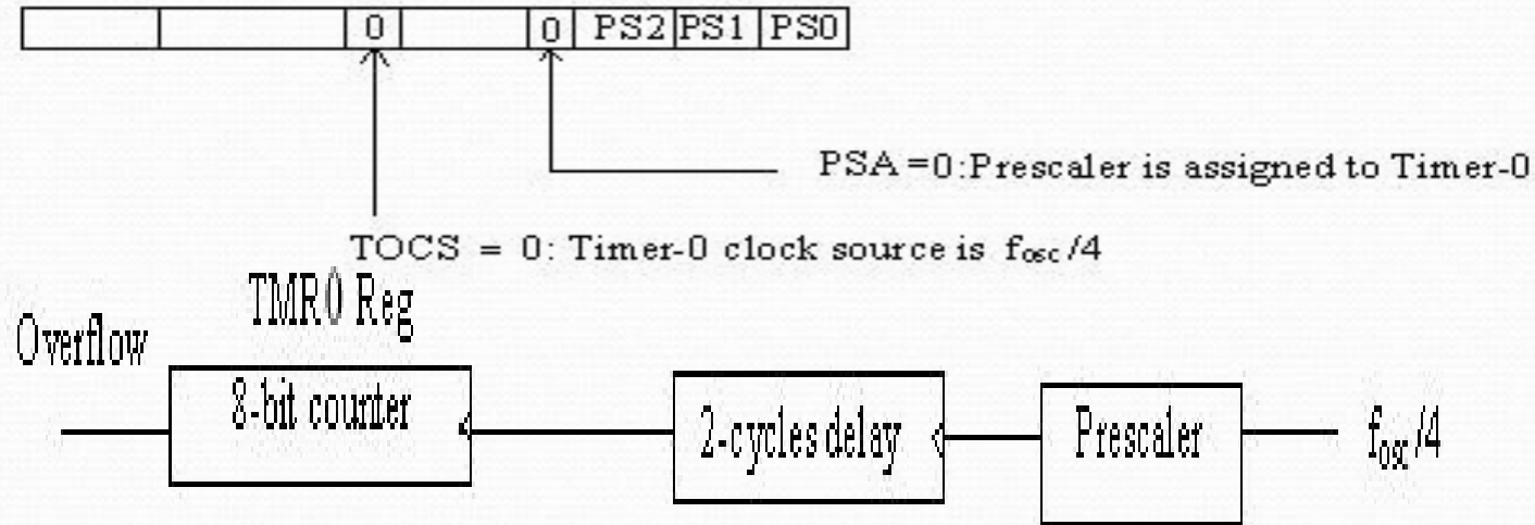
Timer - 0 with prescaler
