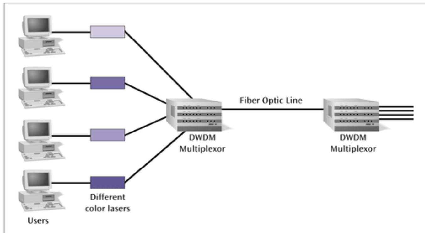
Figure 5-13 Multiple lasers transmitting data signals down a single fiber optic line
