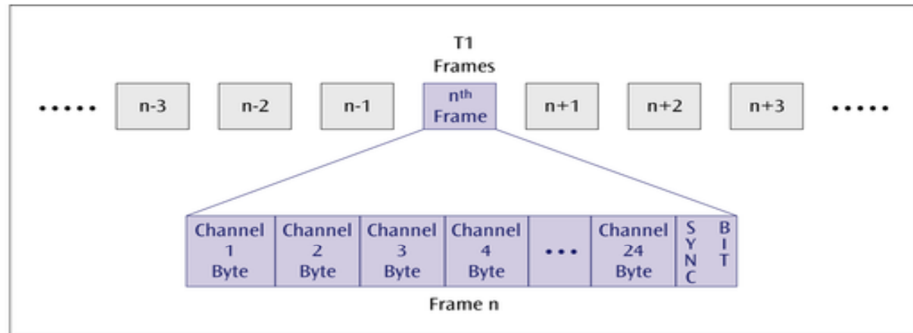
Figure 5-6 T1 multiplexed data stream
