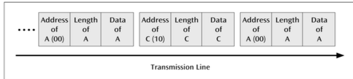
Figure 5-11 Packets of address and data fields in a statistical multiplexor output stream
