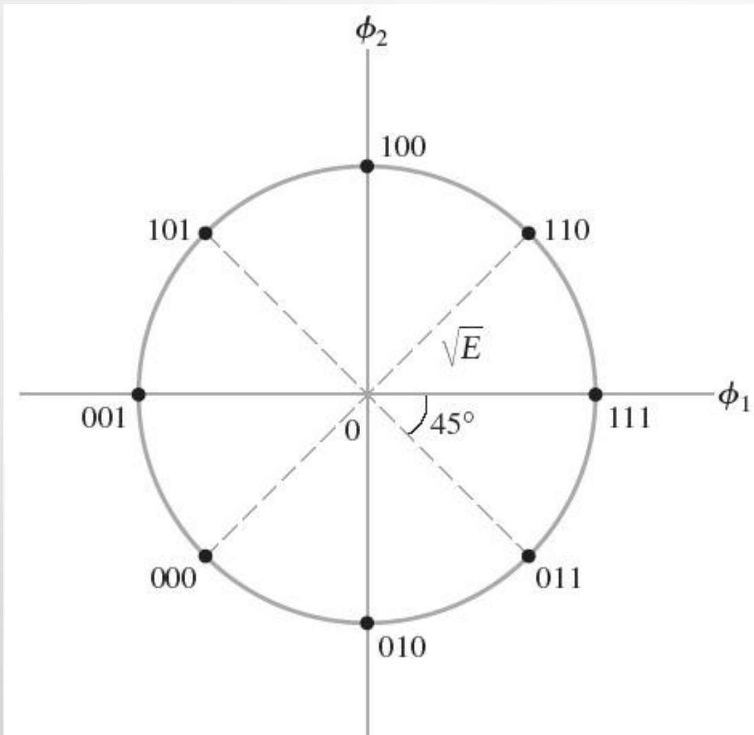
FIGURE 7.20 Signal-space diagram of 8-PSK.
